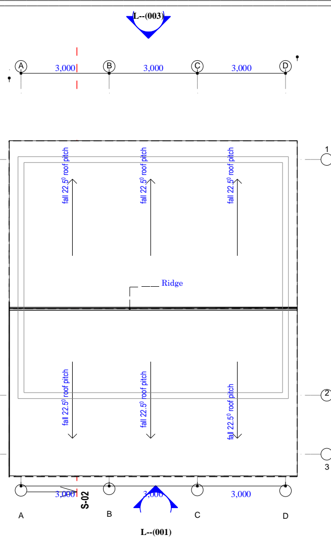
ROOF PLAN
