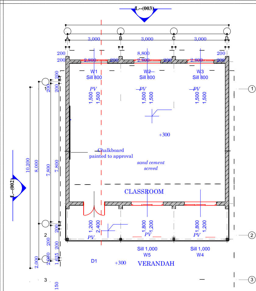
FLOOR PLAN
