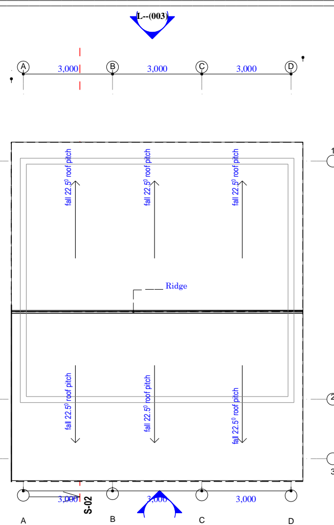
ROOF PLAN
